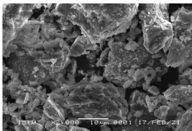
Figure 8 SEM images Ordinary Portland Cement (OPC).
