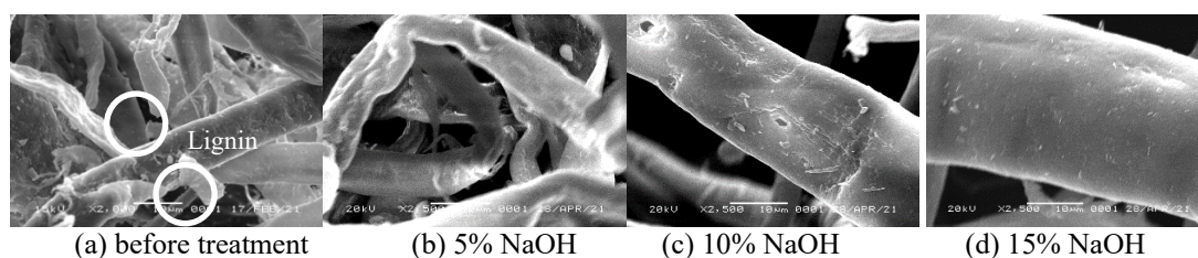
Figure 5 SEM images of treated waste paper in heating temperature 100 °C with (a) before treatment (b) 5 % NaOH, (c) 10 % NaOH, and (d) 15 % NaOH.
