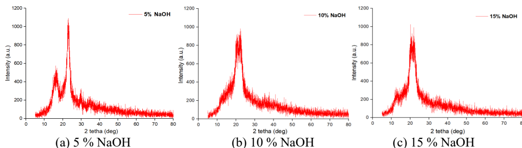
Figure 3 XRD pattern of treated materials in heating temperature 150 °C with (a) 5 % NaOH, (b) 10 % NaOH, and (c) 15 % NaOH.
