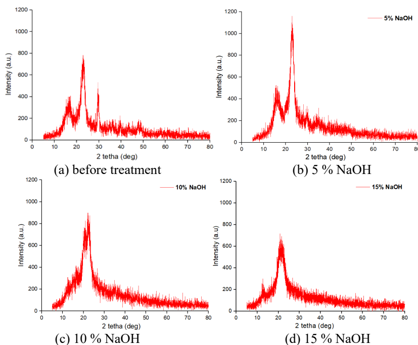
Figure 1 XRD pattern of treated materials in heating temperatures 100 °C with (a) before treatment (b) 5 % NaOH, (c) 10 % NaOH, and (d) 15 % NaOH.
