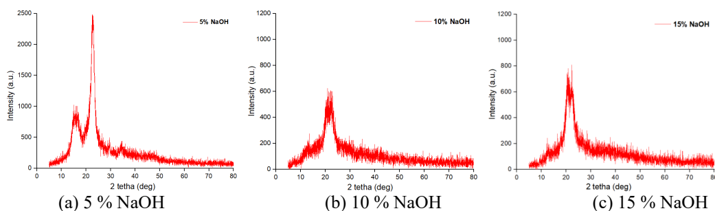
Figure 2 XRD pattern of treated materials in heating temperature 125 °C with (a) 5 % NaOH, (b) 10 % NaOH, and (c) 15 % NaOH.
