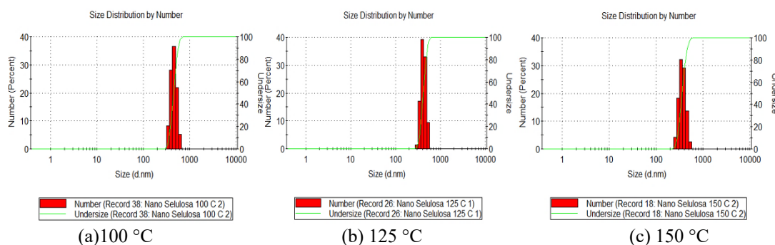
Figure 9 Distribution of particle size nanomaterials with 5 % NaOH at heating temperatures of (a) 100 °C, (b) 125 °C, and (c) 150 °C.
