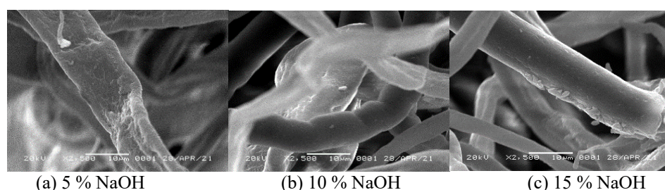
Figure 6 SEM images of treated waste paper in heating temperature 125 °C with (a) 5 % NaOH, (b) 10 % NaOH, and (c) 15 % NaOH.
