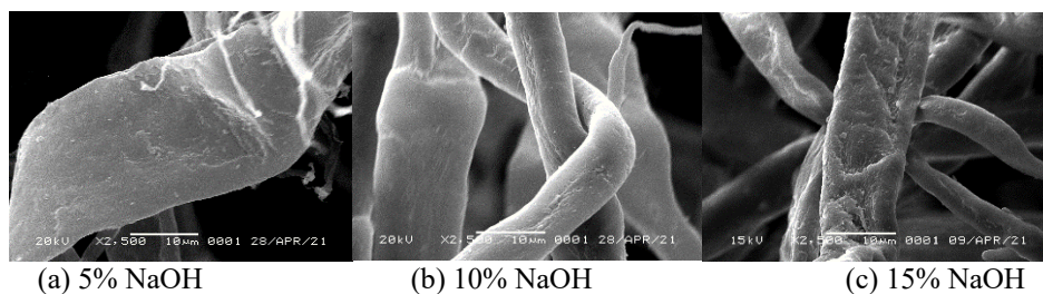
Figure 7 SEM images of treated waste paper in heating temperature 150 °C with (a) 5 % NaOH, (b) 10 % NaOH, and (c) 15 % NaOH.
