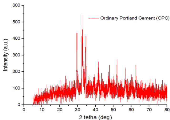
Figure 4 XRD patterns of Ordinary Portland Cement.
