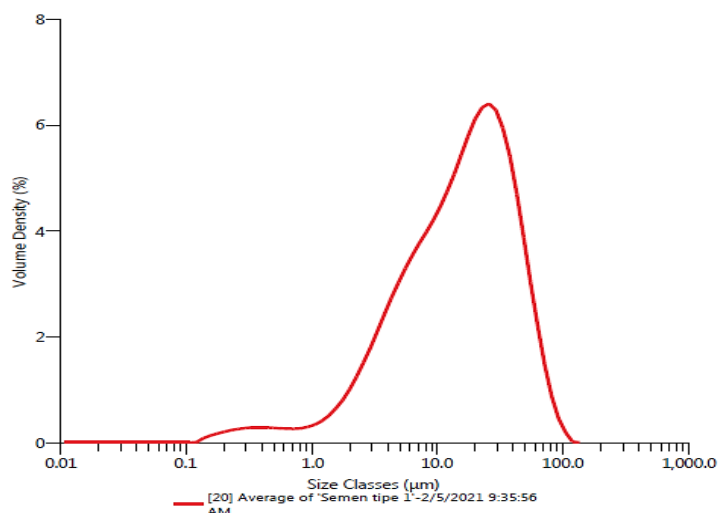
Figure 10 Distribution of particle size OPC.
