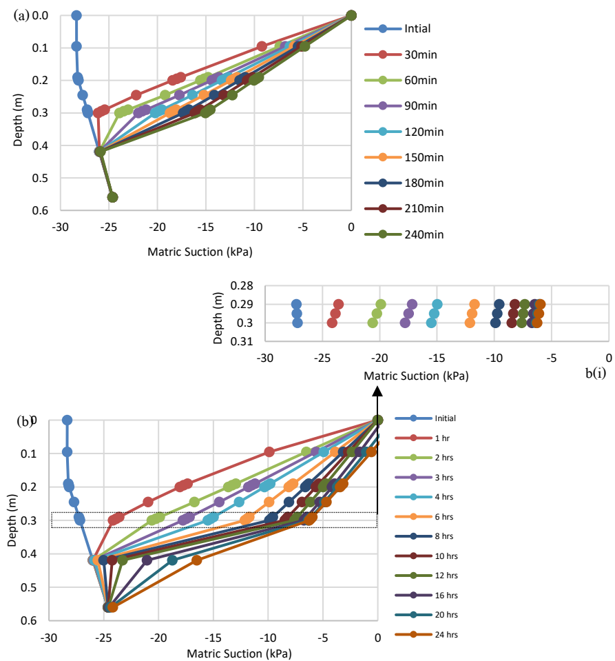
Figure 4 Suction distribution for clayey silt and gravelly silt without porous transport layer due to (a) 4 h and (b) 24 h rainfall pattern.
