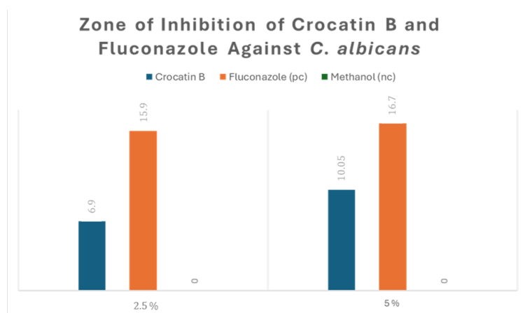
Figure 3 Zone of inhibition (mm) of crocacin B and Fluconazole against C. albicans .
