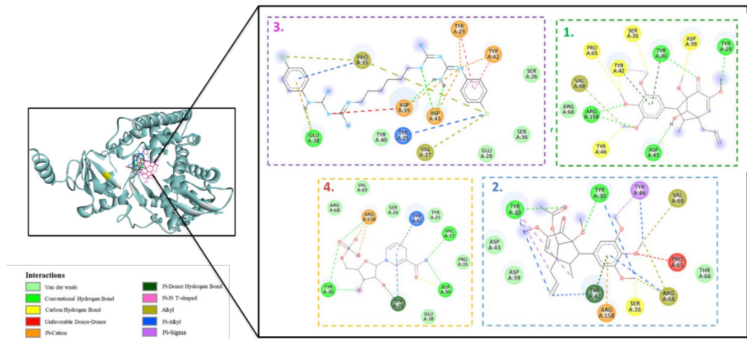
Figure 4 Molecular Interaction of (1) crocatin B, (2) crocatin A, (3) chlorhexidine and (4) native ligand to DNA ligase Enzyme.
